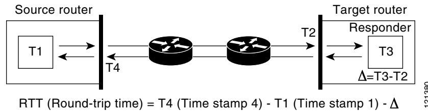
Figure 38-2 Cisco IOS IP SLAs Responder Time Stamping
