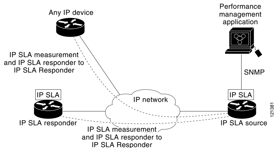
Figure 38-1 Cisco IOS IP SLAs Operation
